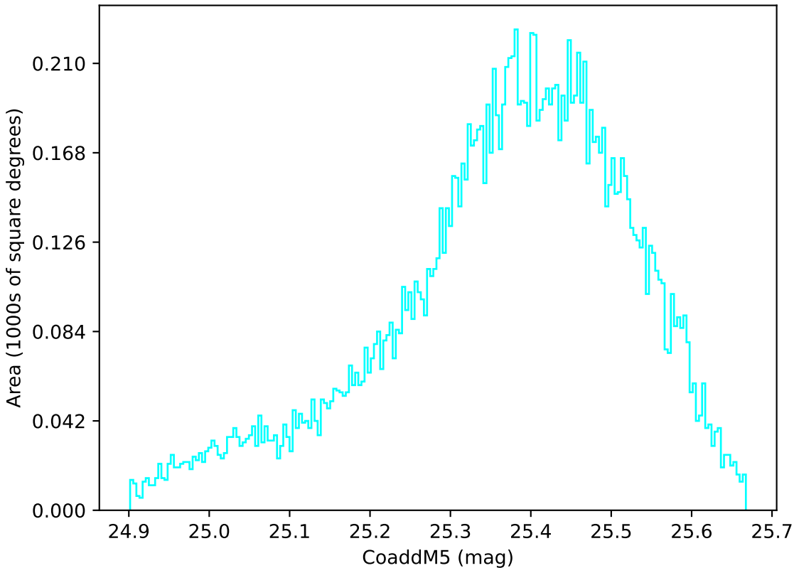
too_elab_r128_d3_gz_v3.4_10yrs WFD u band: CoaddM5
