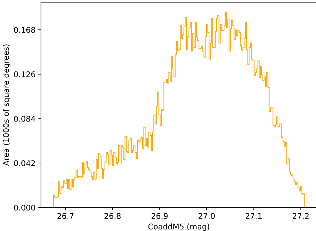
too_elab_r128_d3_gz_v3.4_10yrs WFD r band: CoaddM5
