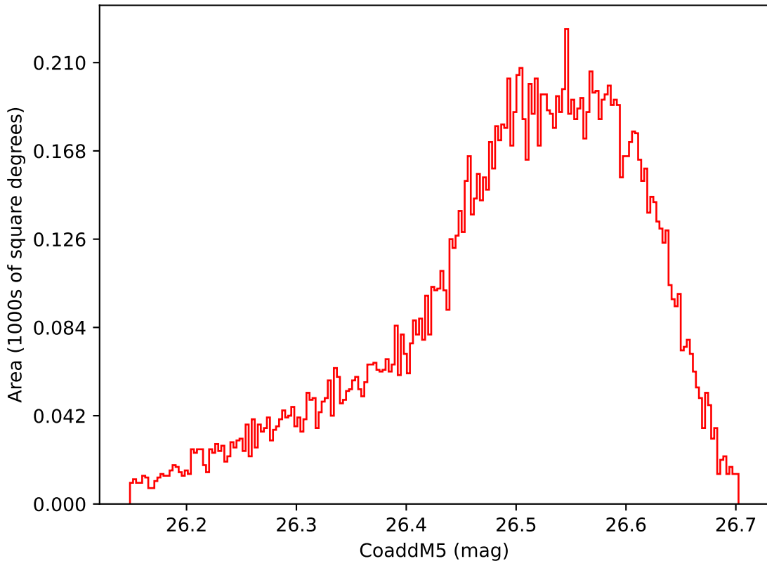
too_elab_r128_d3_gz_v3.4_10yrs WFD i band: CoaddM5
