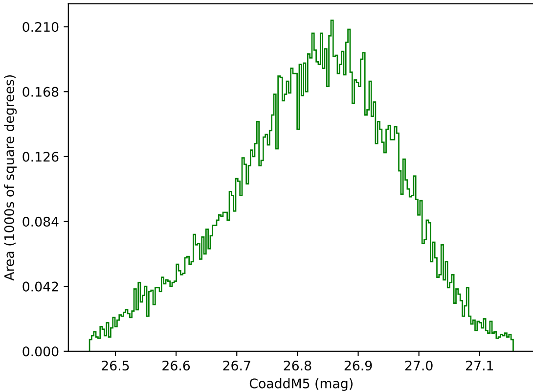
too_elab_r128_d3_gz_v3.4_10yrs WFD g band: CoaddM5
