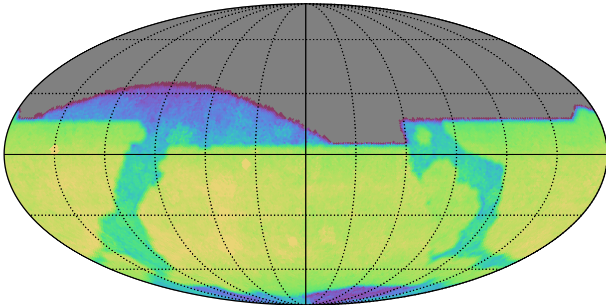
too_elab_r128_d3_gz_v3.4_10yrs All sky z band: CoaddM5
