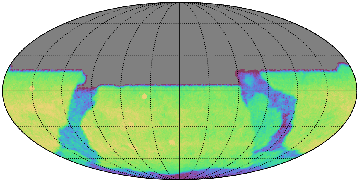
too_elab_r128_d3_gz_v3.4_10yrs All sky u band: CoaddM5
