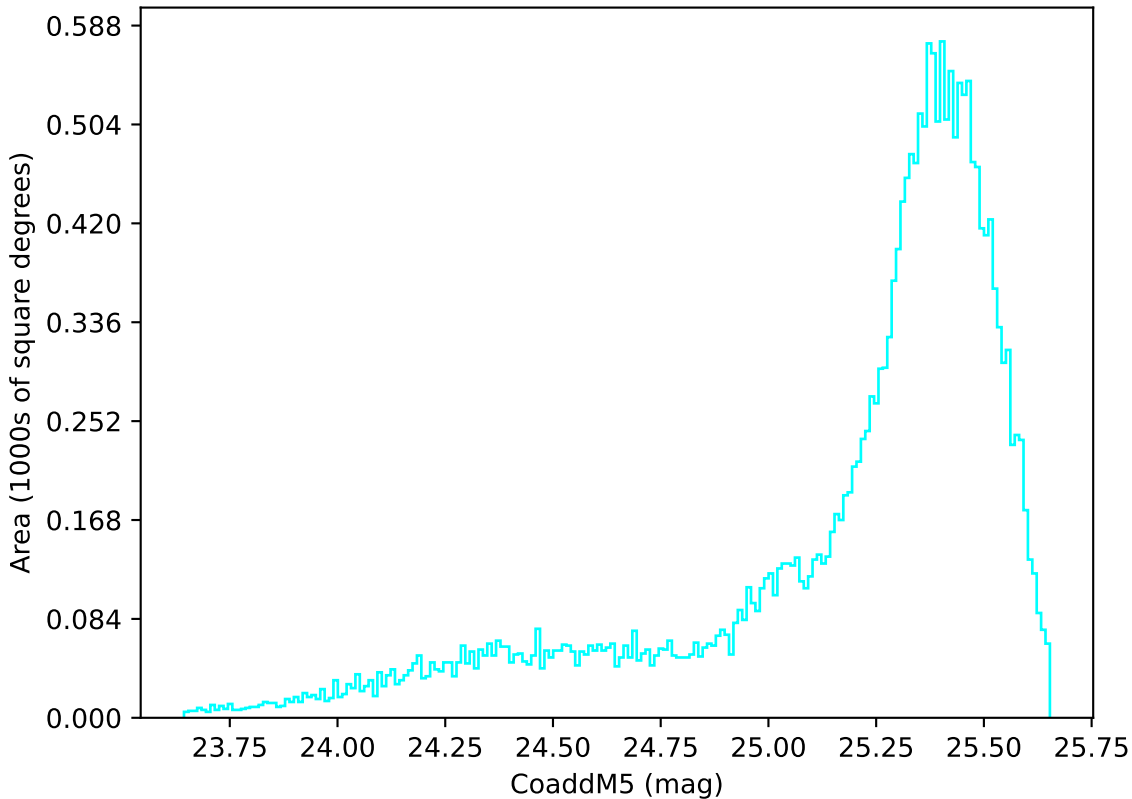
too_elab_r128_d3_gz_v3.4_10yrs All sky u band: CoaddM5
