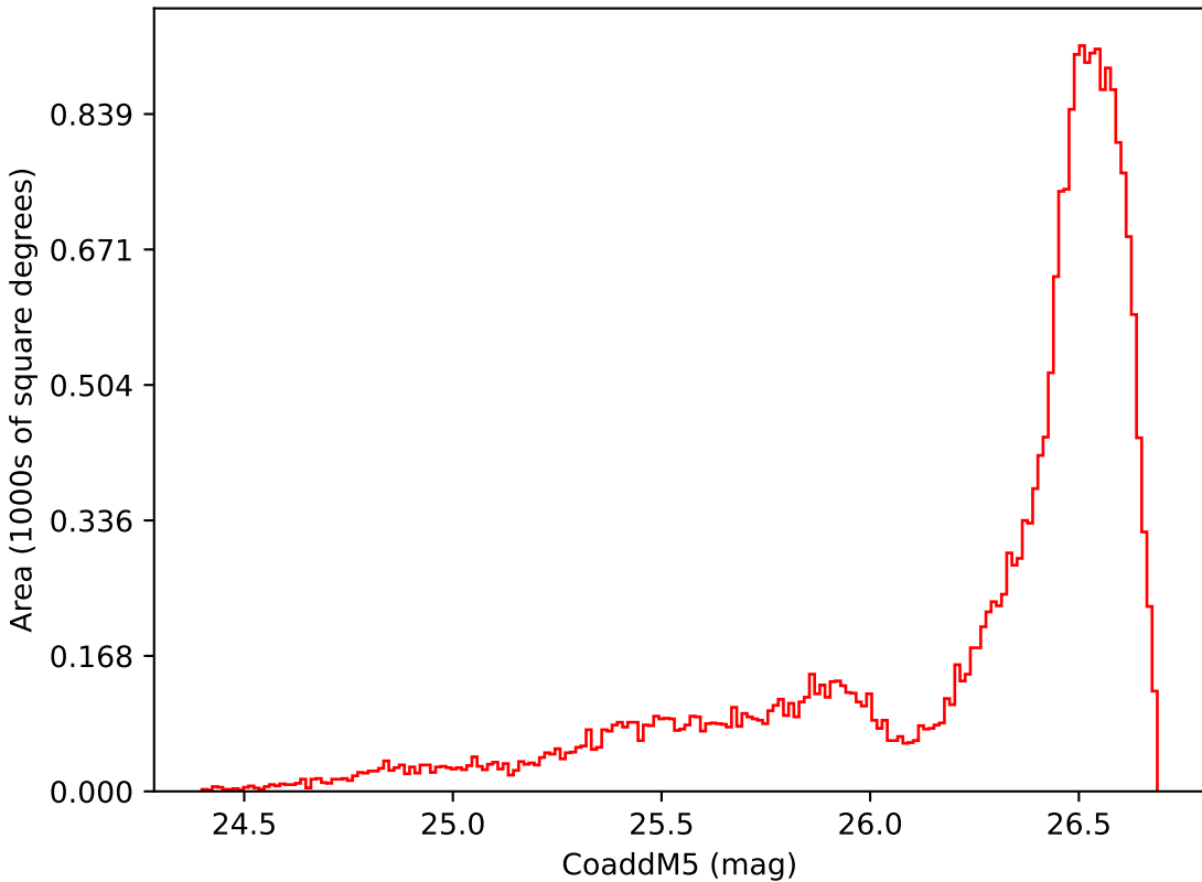
too_elab_r128_d3_gz_v3.4_10yrs All sky i band: CoaddM5
