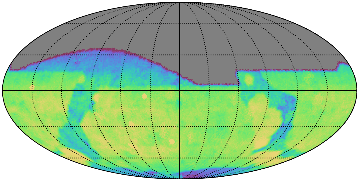
too_elab_r128_d3_gz_v3.4_10yrs All sky g band: CoaddM5
