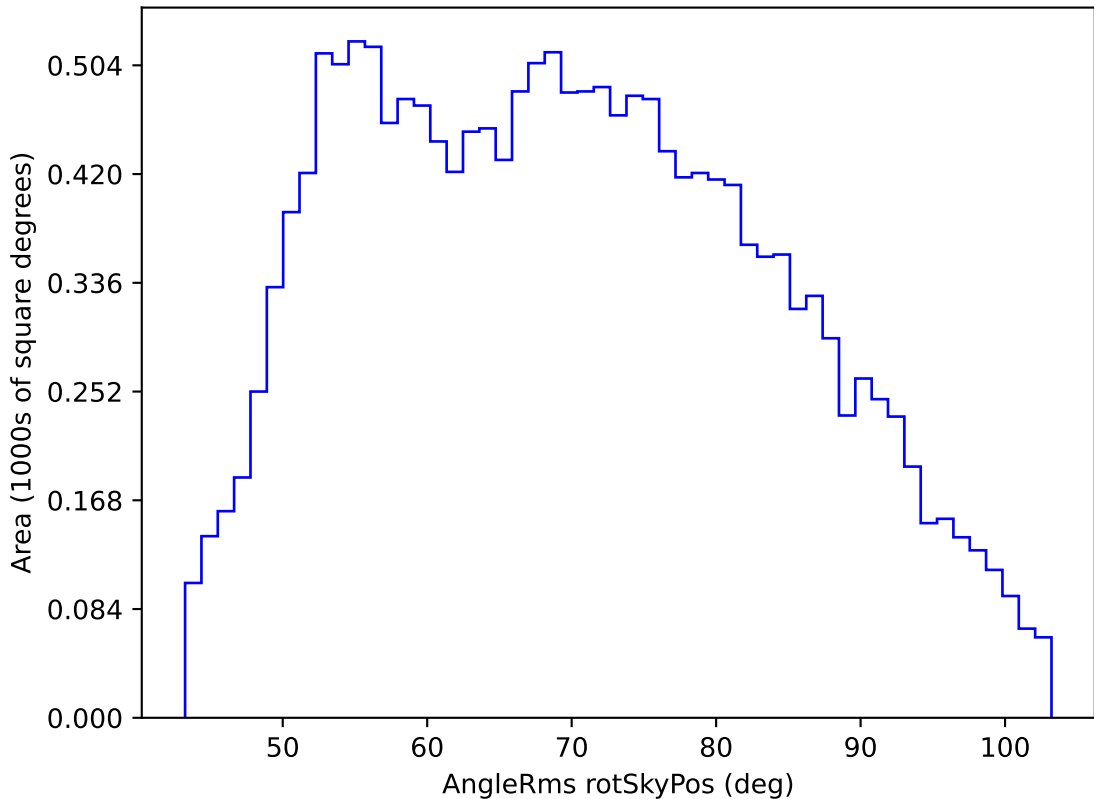
too_elab_r128_d3_gz_v3.4_10yrs WFD g band: AngleRms rotSkyPos
