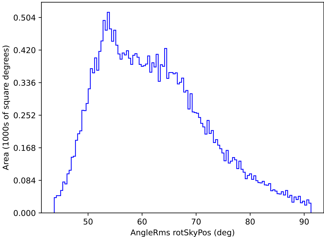
too_elab_r128_d3_gz_v3.4_10yrs All sky i band: AngleRms rotSkyPos
