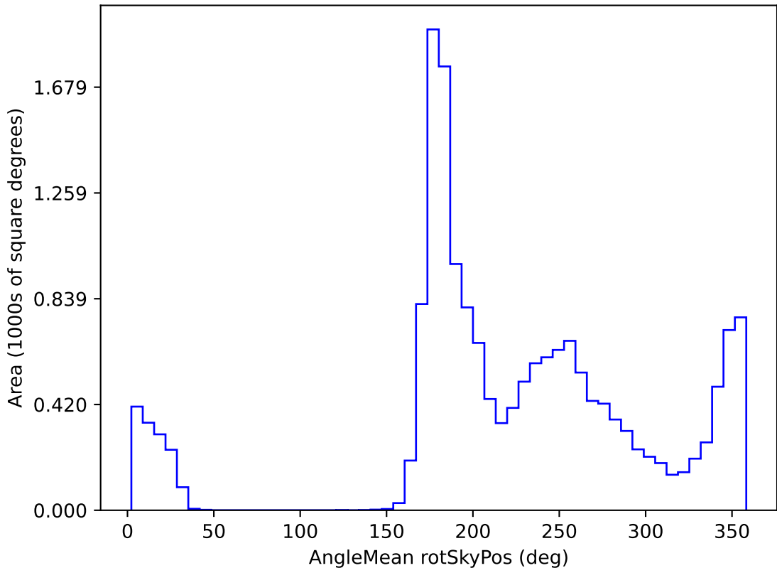
too_elab_r128_d3_gz_v3.4_10yrs WFD i band: AngleMean rotSkyPos
