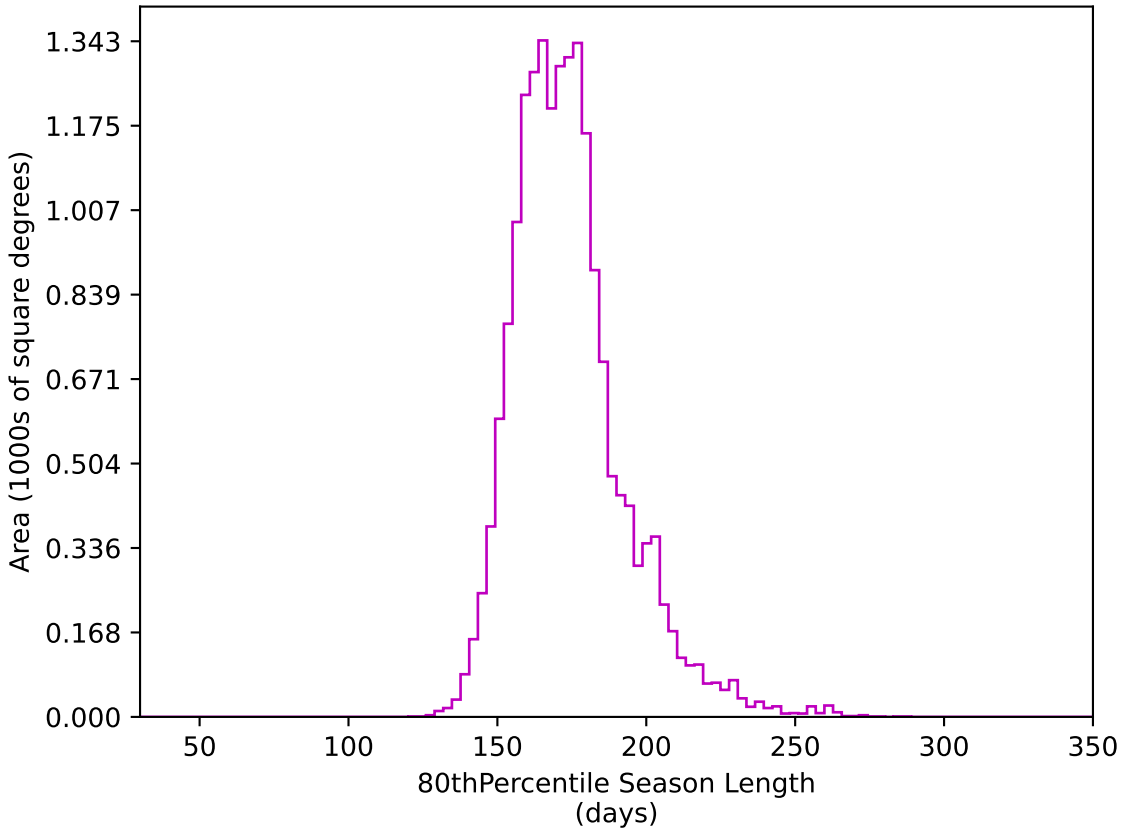
too_elab_r128_d3_gz_v3.4_10yrs WFD z band: 80thPercentile Season Length
