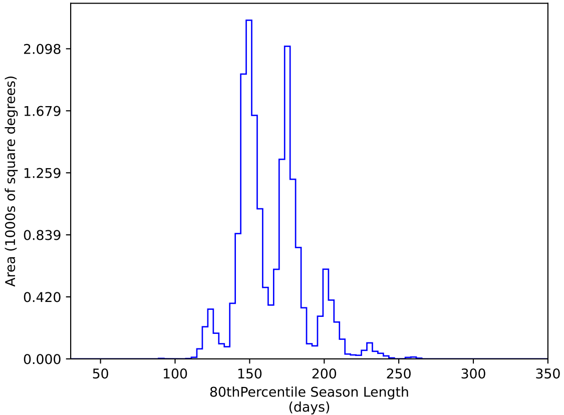
too_elab_r128_d3_gz_v3.4_10yrs WFD y band: 80thPercentile Season Length
