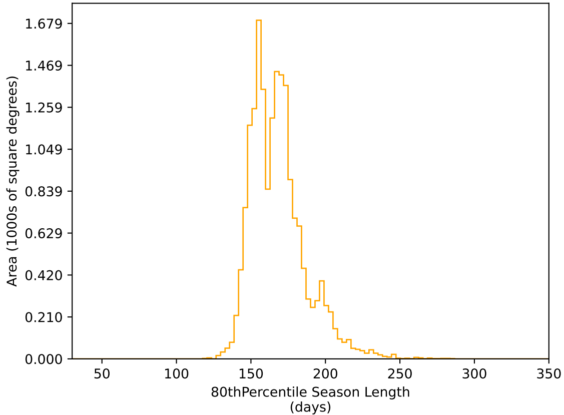
too_elab_r128_d3_gz_v3.4_10yrs WFD r band: 80thPercentile Season Length
