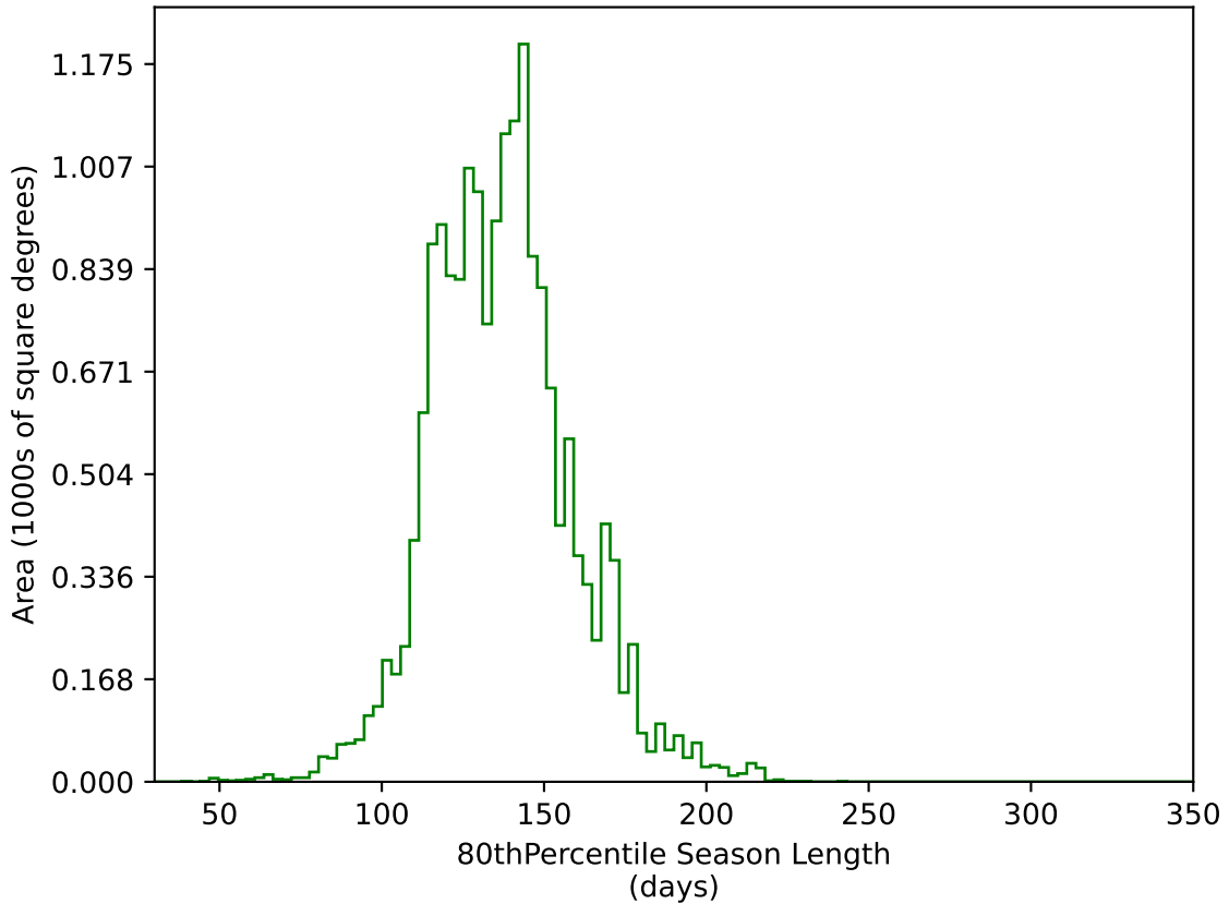
too_elab_r128_d3_gz_v3.4_10yrs WFD g band: 80thPercentile Season Length
