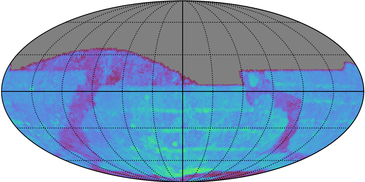
too_elab_r128_d3_gz_v3.4_10yrs All sky z band: 80thPercentile Season Length
