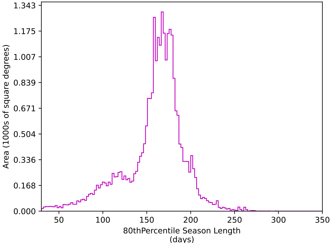
too_elab_r128_d3_gz_v3.4_10yrs All sky z band: 80thPercentile Season Length
