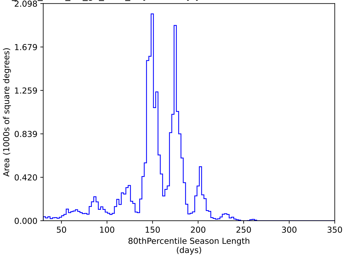
too_elab_r128_d3_gz_v3.4_10yrs All sky y band: 80thPercentile Season Length
