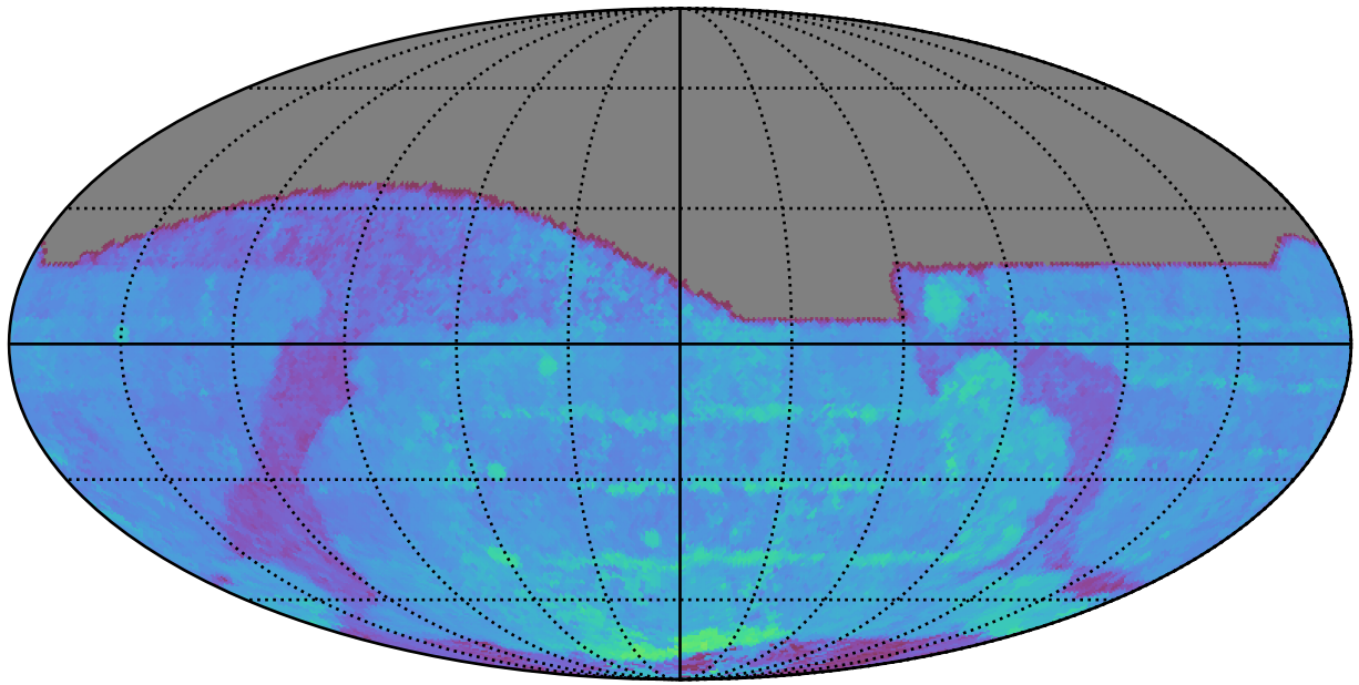
too_elab_r128_d3_gz_v3.4_10yrs All sky i band: 80thPercentile Season Length
