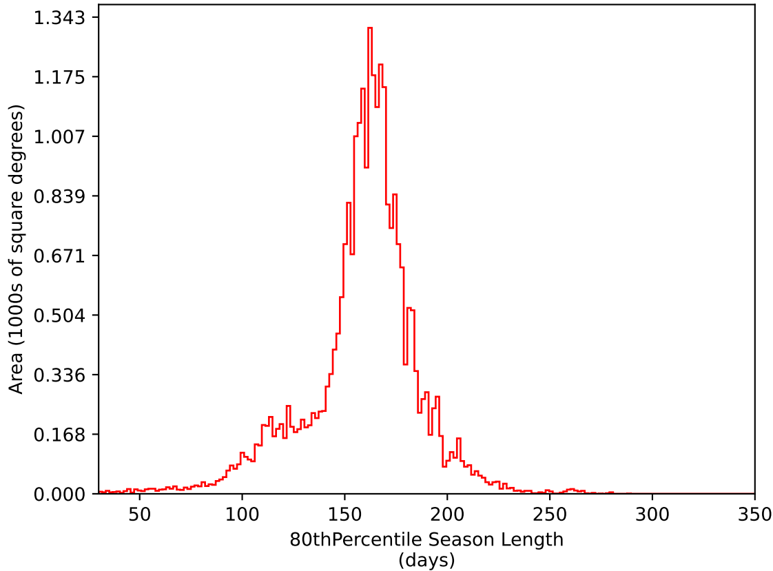
too_elab_r128_d3_gz_v3.4_10yrs All sky i band: 80thPercentile Season Length
