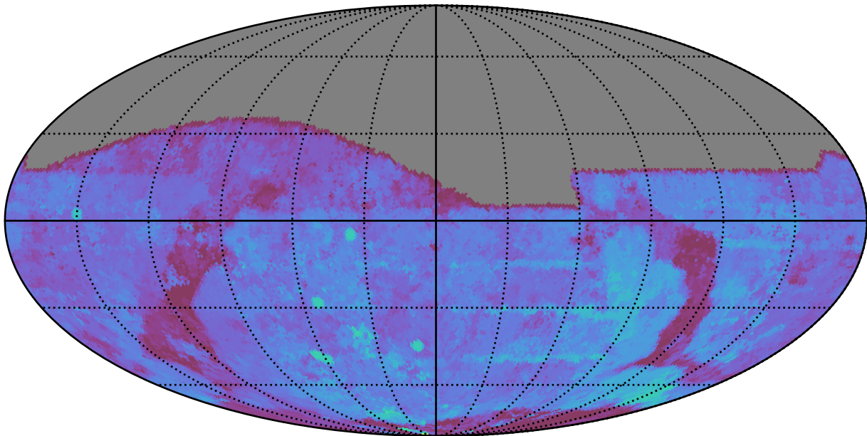
too_elab_r128_d3_gz_v3.4_10yrs All sky g band: 80thPercentile Season Length
