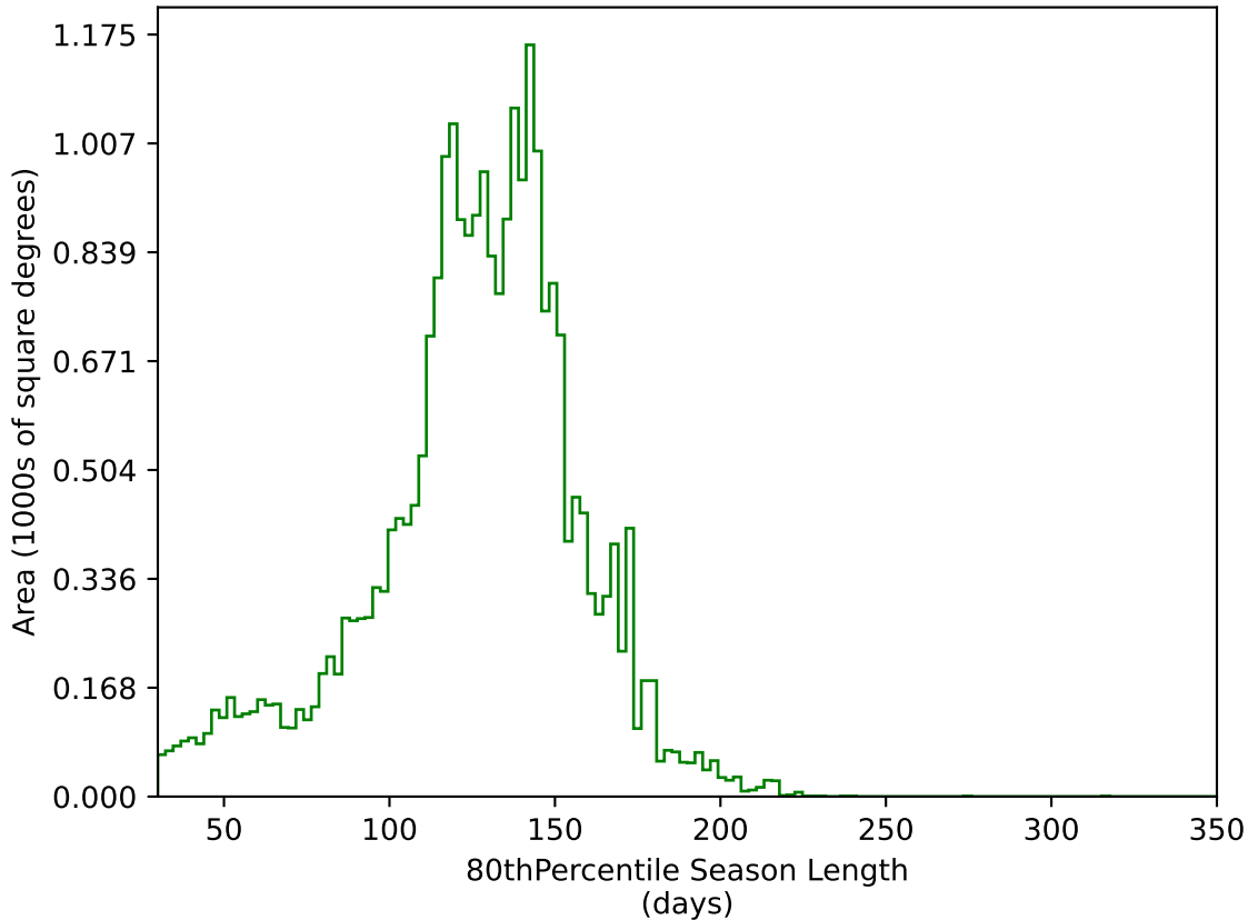
too_elab_r128_d3_gz_v3.4_10yrs All sky g band: 80thPercentile Season Length
