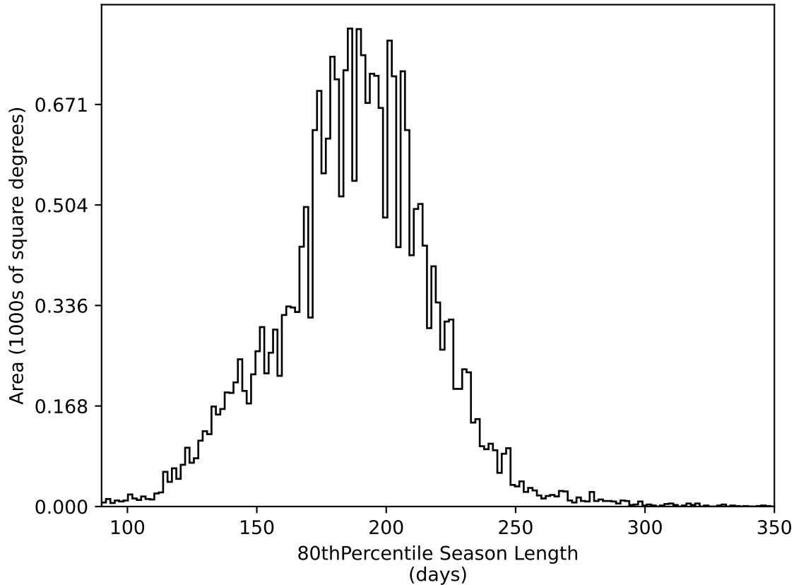
too_elab_r128_d3_gz_v3.4_10yrs All sky all bands: 80thPercentile Season Length
