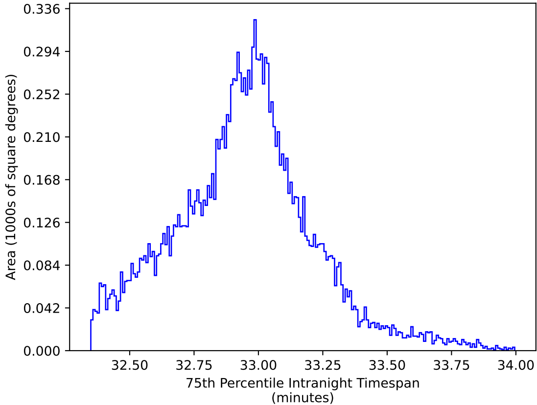
too_elab_r128_d3_gz_v3.4_10yrs WFD y band: 75th Percentile Intranight Timespan
