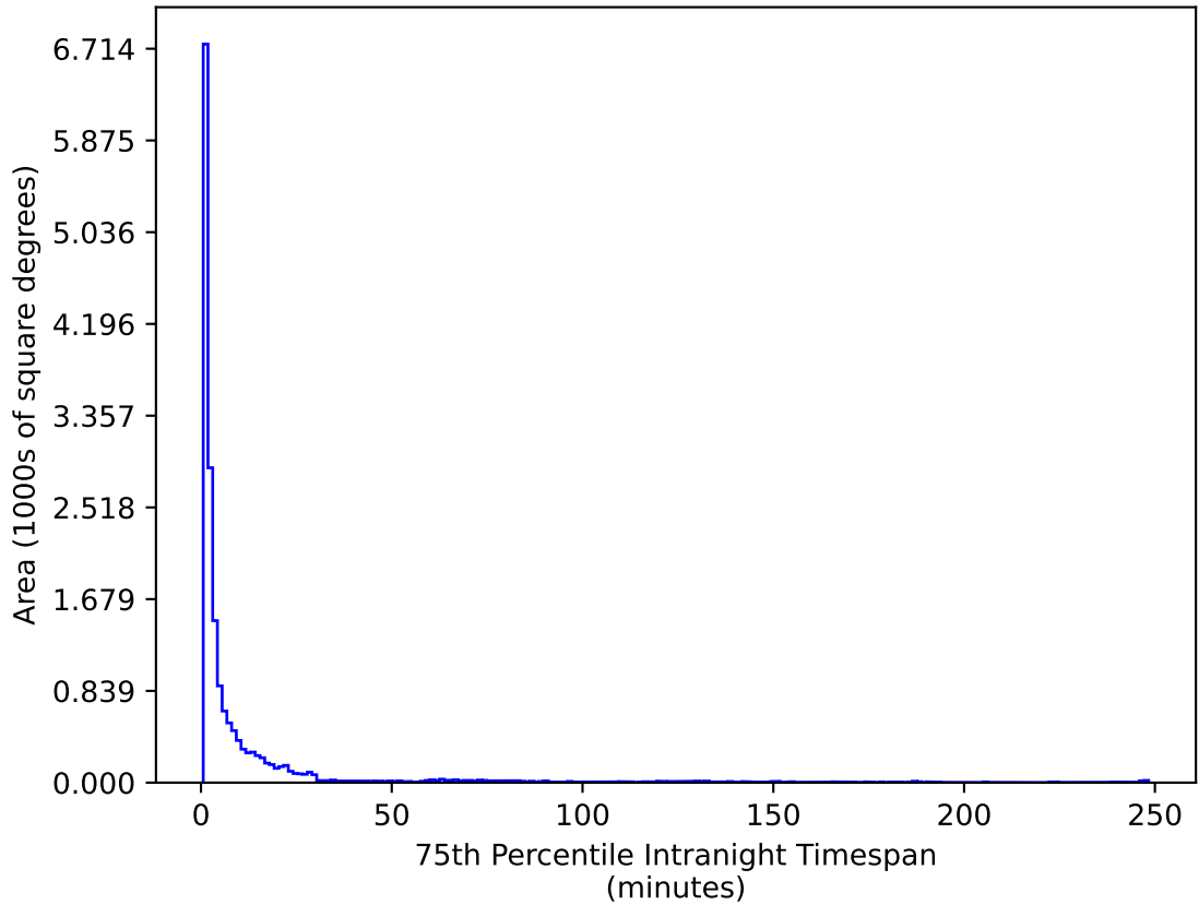
too_elab_r128_d3_gz_v3.4_10yrs WFD u band: 75th Percentile Intranight Timespan
