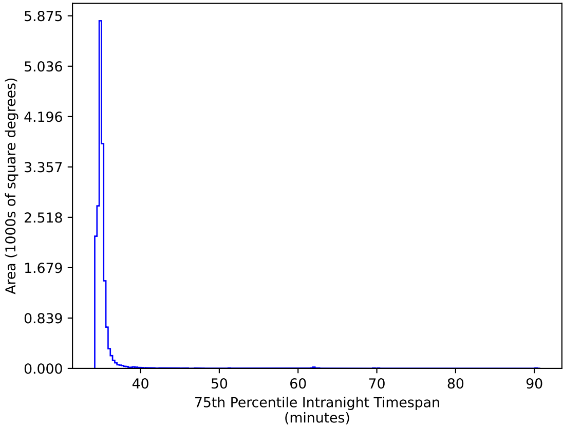
too_elab_r128_d3_gz_v3.4_10yrs WFD ri bands: 75th Percentile Intranight Timespan
