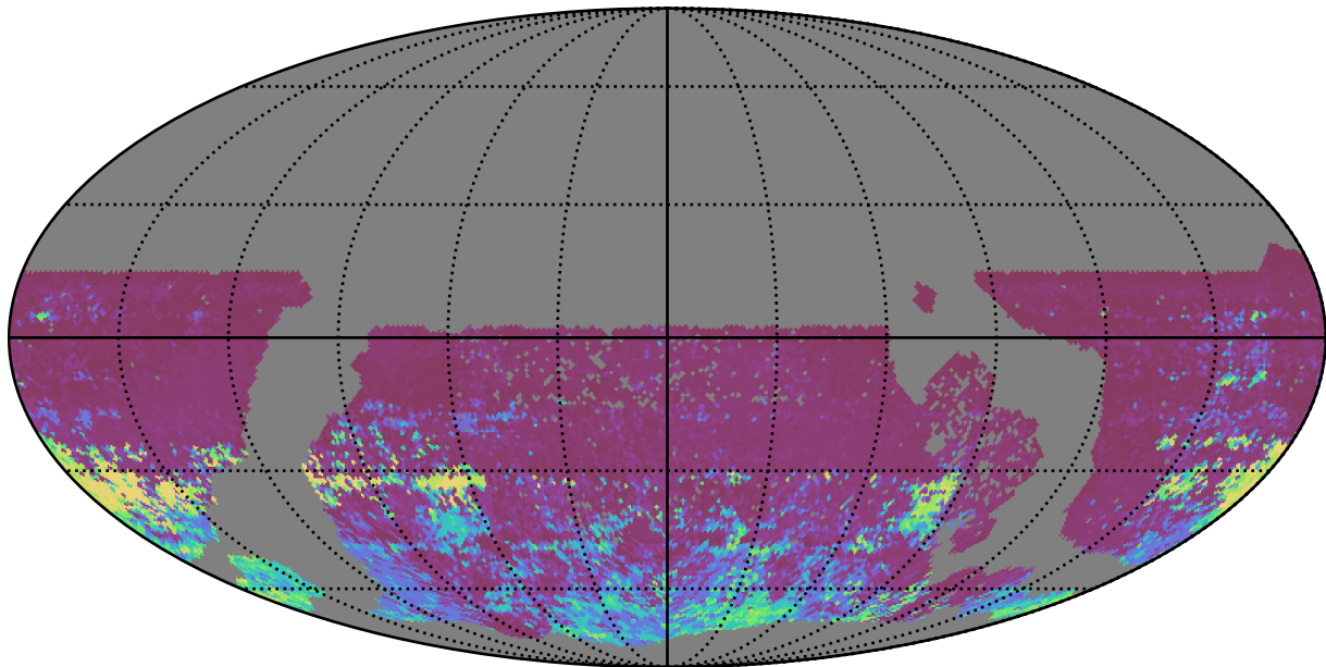
too_elab_r128_d3_gz_v3.4_10yrs WFD r band: 75th Percentile Intranight Timespan
