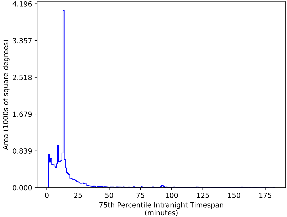
too_elab_r128_d3_gz_v3.4_10yrs WFD i band: 75th Percentile Intranight Timespan
