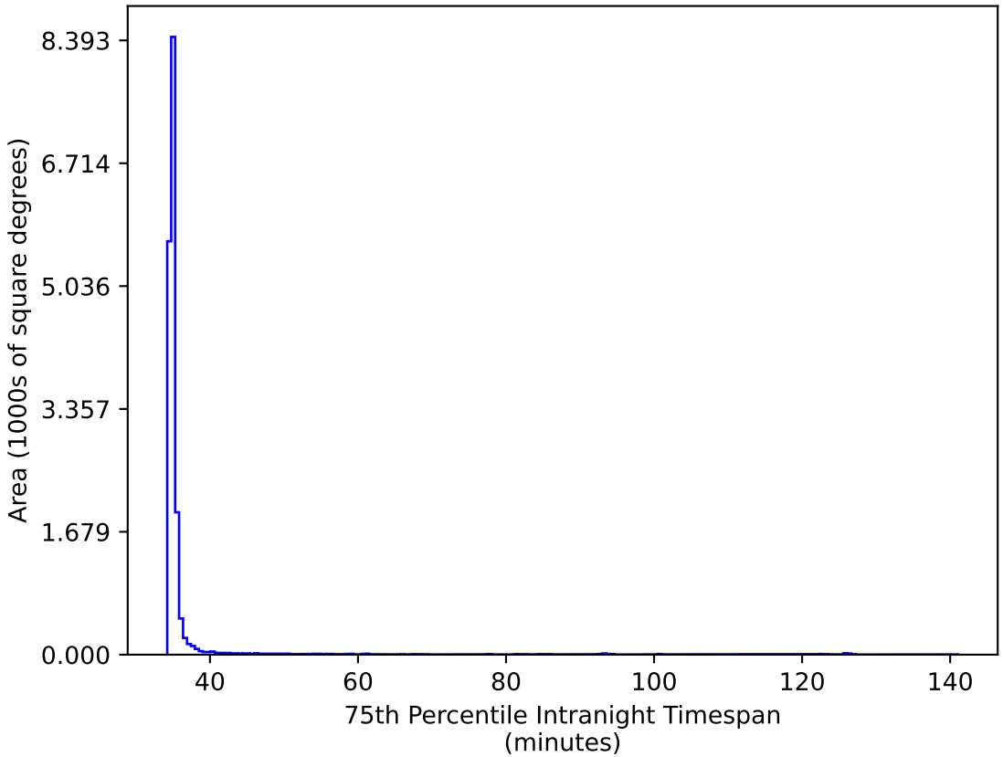
too_elab_r128_d3_gz_v3.4_10yrs WFD gr bands: 75th Percentile Intranight Timespan
