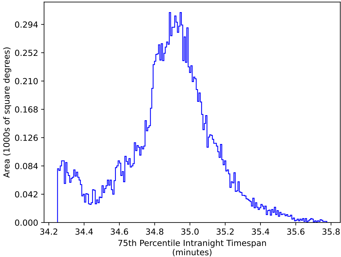
too_elab_r128_d3_gz_v3.4_10yrs WFD: 75th Percentile Intranight Timespan
