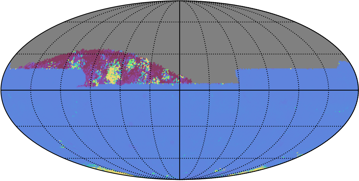
too_elab_r128_d3_gz_v3.4_10yrs All sky zy bands: 75th Percentile Intranight Timespan
