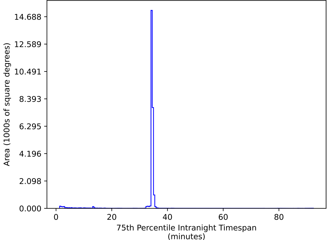
too_elab_r128_d3_gz_v3.4_10yrs All sky zy bands: 75th Percentile Intranight Timespan
