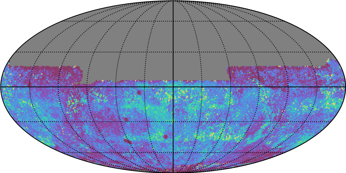
too_elab_r128_d3_gz_v3.4_10yrs All sky y band: 75th Percentile Intranight Timespan
