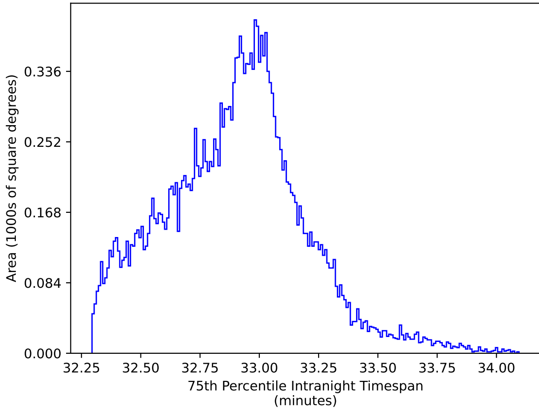
too_elab_r128_d3_gz_v3.4_10yrs All sky y band: 75th Percentile Intranight Timespan
