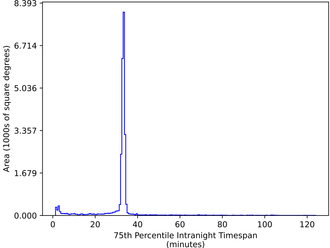
too_elab_r128_d3_gz_v3.4_10yrs All sky ug bands: 75th Percentile Intranight Timespan
