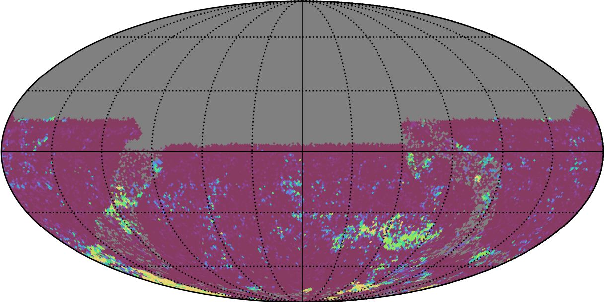
too_elab_r128_d3_gz_v3.4_10yrs All sky u band: 75th Percentile Intranight Timespan
