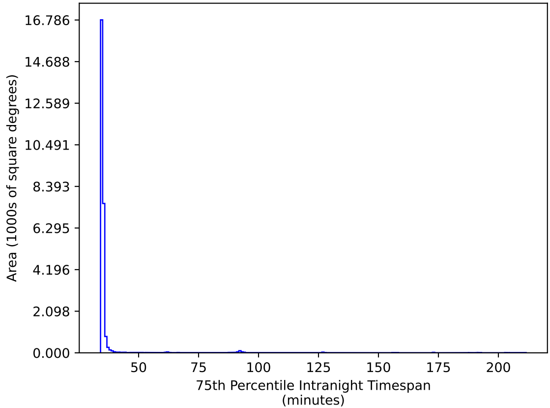
too_elab_r128_d3_gz_v3.4_10yrs All sky ri bands: 75th Percentile Intranight Timespan
