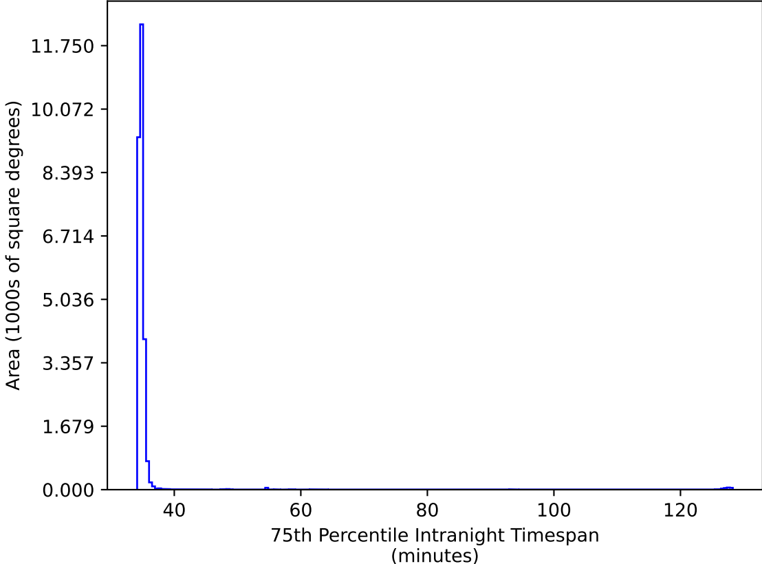
too_elab_r128_d3_gz_v3.4_10yrs All sky iz bands: 75th Percentile Intranight Timespan
