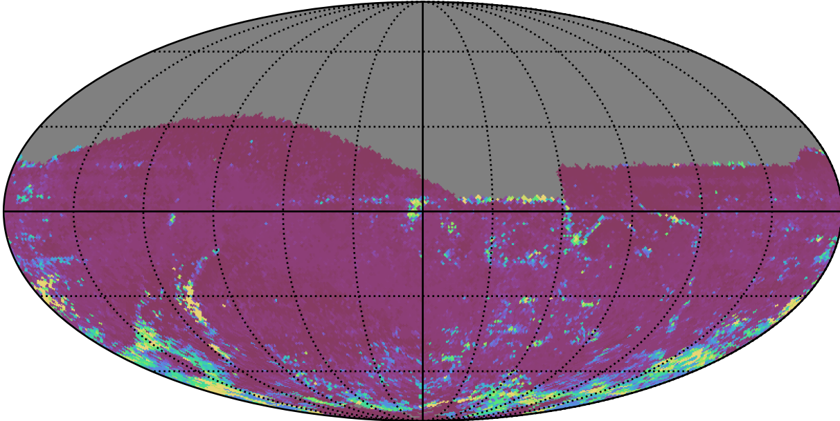
too_elab_r128_d3_gz_v3.4_10yrs All sky i band: 75th Percentile Intranight Timespan
