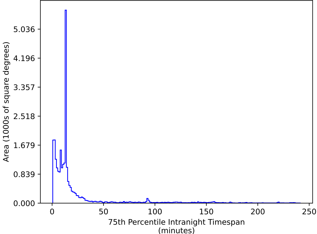
too_elab_r128_d3_gz_v3.4_10yrs All sky i band: 75th Percentile Intranight Timespan
