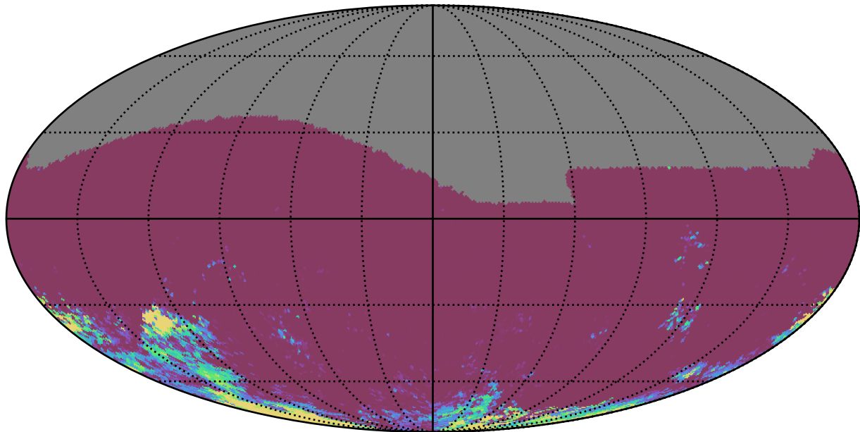
too_elab_r128_d3_gz_v3.4_10yrs All sky gr bands: 75th Percentile Intranight Timespan
