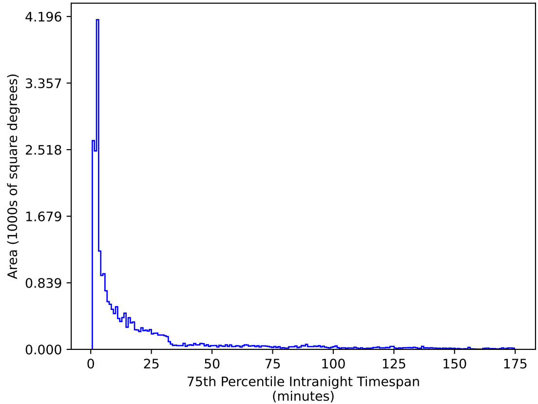
too_elab_r128_d3_gz_v3.4_10yrs All sky g band: 75th Percentile Intranight Timespan
