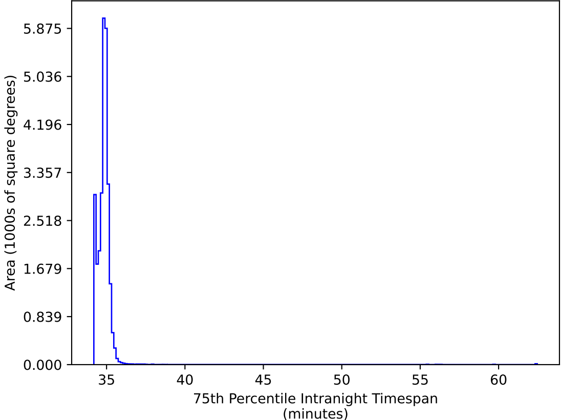
too_elab_r128_d3_gz_v3.4_10yrs All sky all bands: 75th Percentile Intranight Timespan
