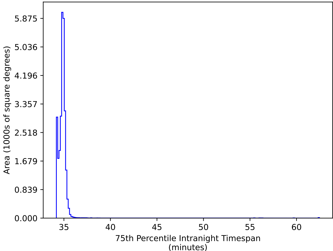
too_elab_r128_d3_gz_v3.4_10yrs All sky: 75th Percentile Intranight Timespan
