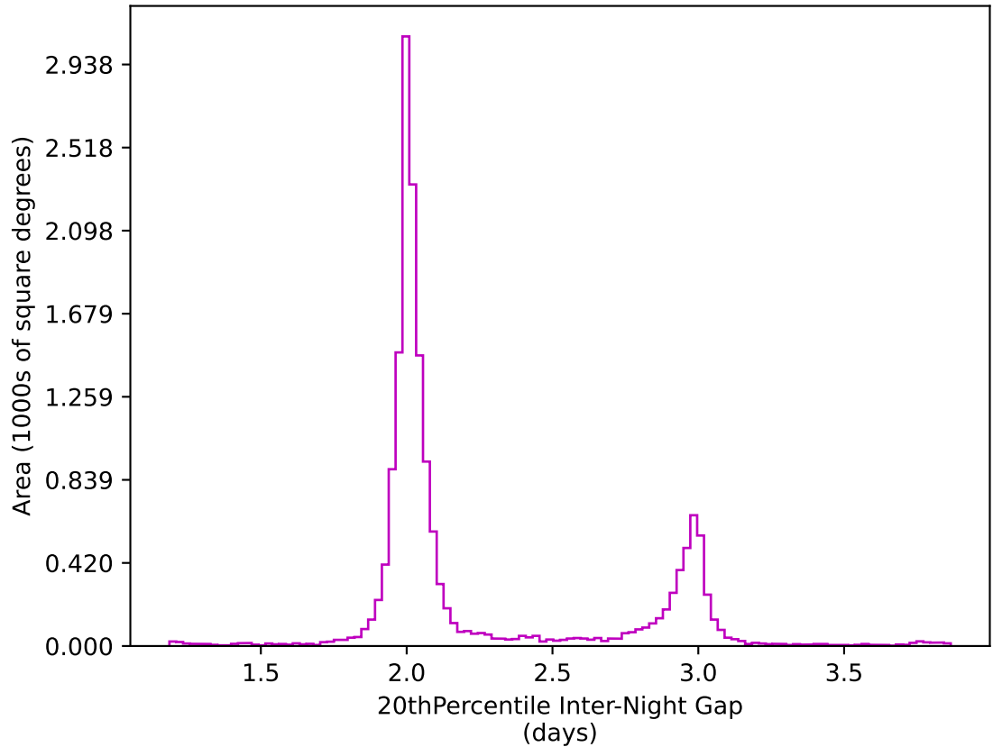
too_elab_r128_d3_gz_v3.4_10yrs WFD z band: 20thPercentile Inter-Night Gap
