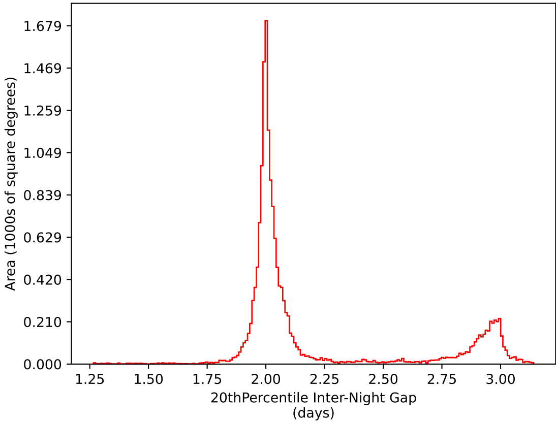
too_elab_r128_d3_gz_v3.4_10yrs WFD i band: 20thPercentile Inter-Night Gap
