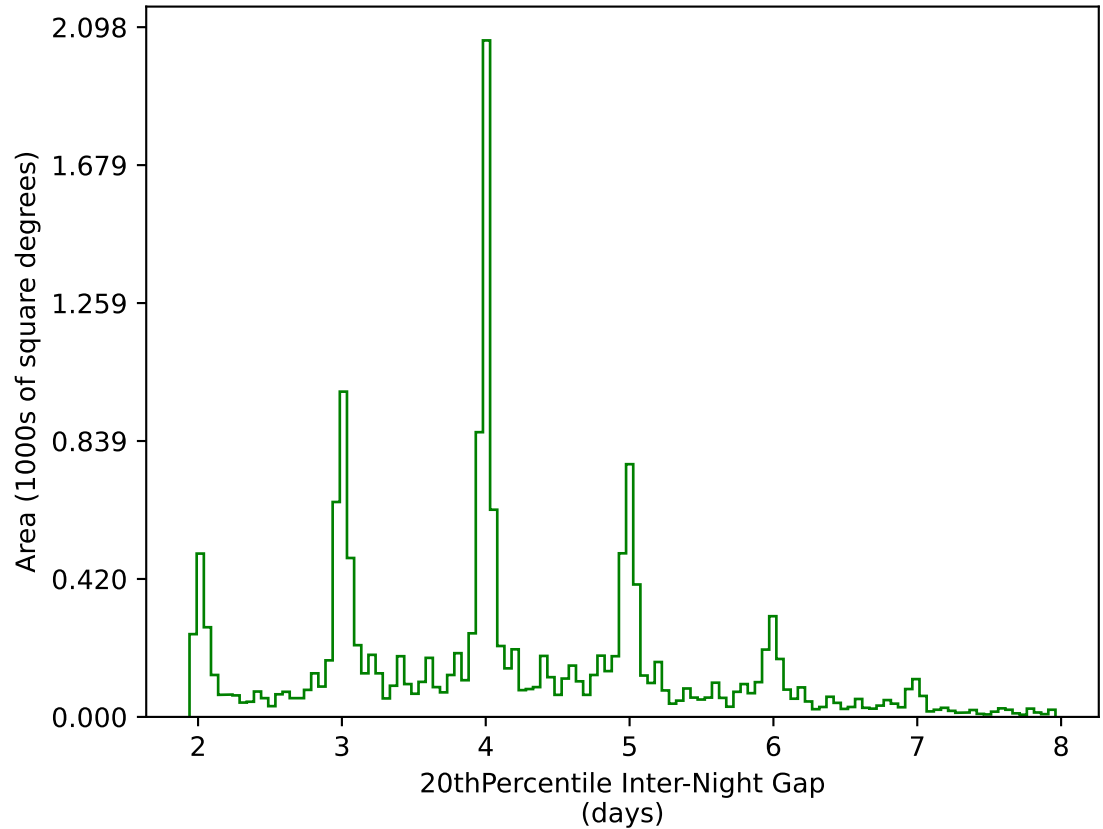
too_elab_r128_d3_gz_v3.4_10yrs WFD g band: 20thPercentile Inter-Night Gap
