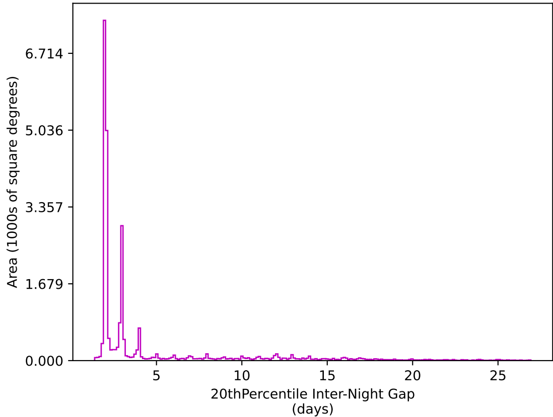
too_elab_r128_d3_gz_v3.4_10yrs All sky z band: 20thPercentile Inter-Night Gap
