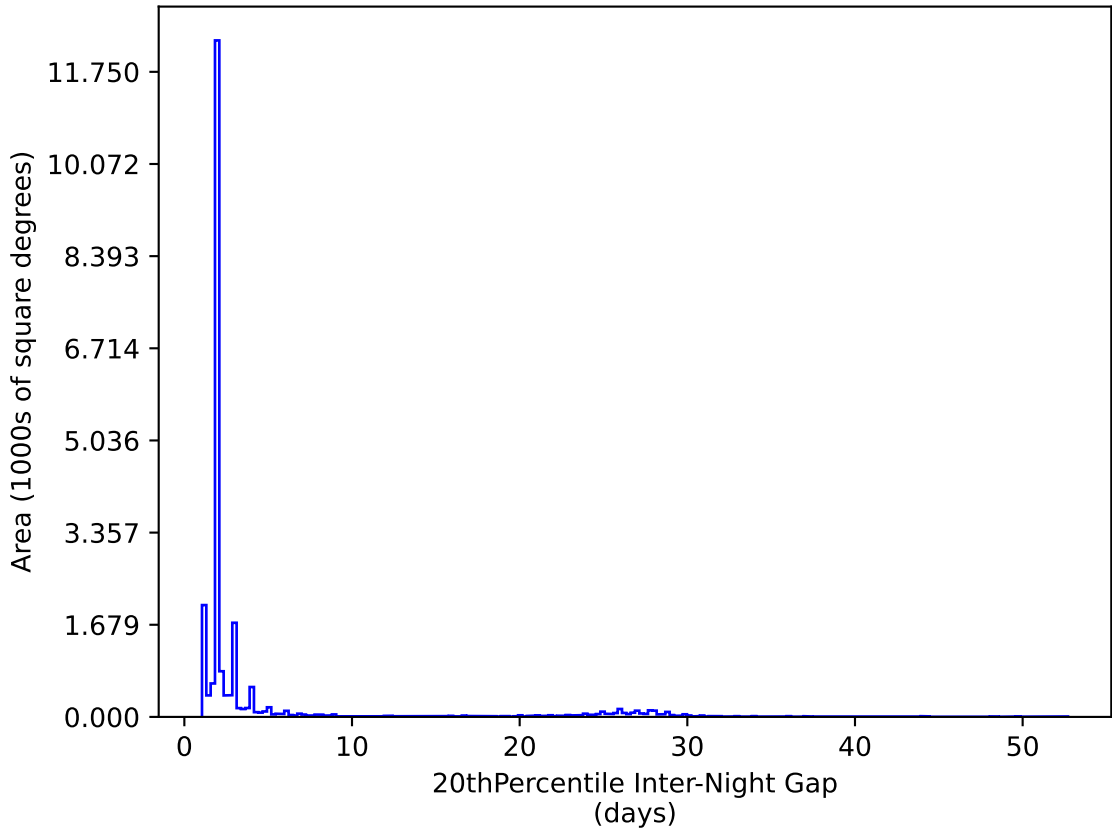
too_elab_r128_d3_gz_v3.4_10yrs All sky y band: 20thPercentile Inter-Night Gap
